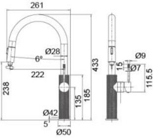
WT 7566 TIARA Sink Mixer With Pull Out Spray WELS: 5 star 6L/min WELS Reg. T41760
