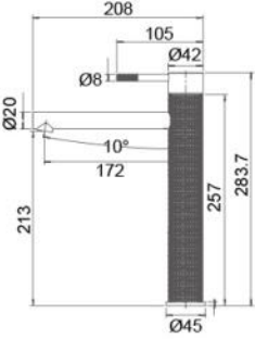
WT 7502 TIARA Tower Basin Mixer WELS: 6 star 4.5L/min WELS Reg. NO.: T41376
