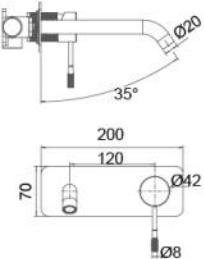
WT 7507 TIARA Wall Basin/Bath Set WELS: 6 star 4.5L/min WELS Reg. NO.: T41339
